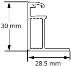
LONG SIDE FRAME PROFILE
