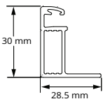
LONG SIDE FRAME PROFILE
