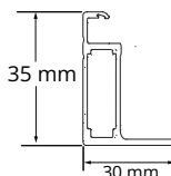
SIDE FRAME PROFILE
